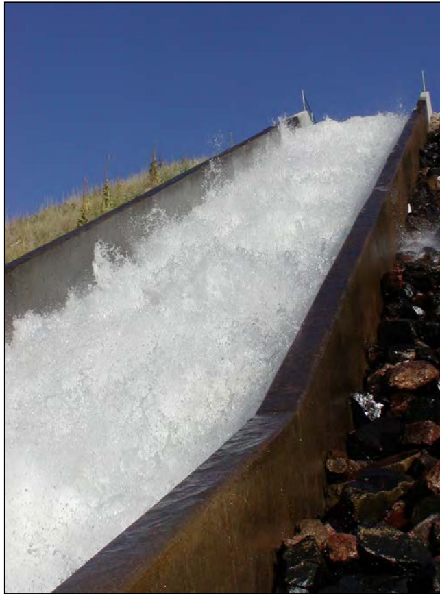
Figure 140.—Baffled drop aerating the flow so that it becomes saturated.
