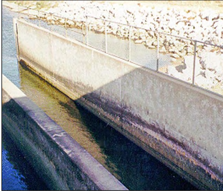
Figure A-120.—Close-up of right wall of river outlet works stilling basin. Arrows denote area of staining from hydraulic jump which roughly corresponds to area with exposed reinforcing steel in floor.
