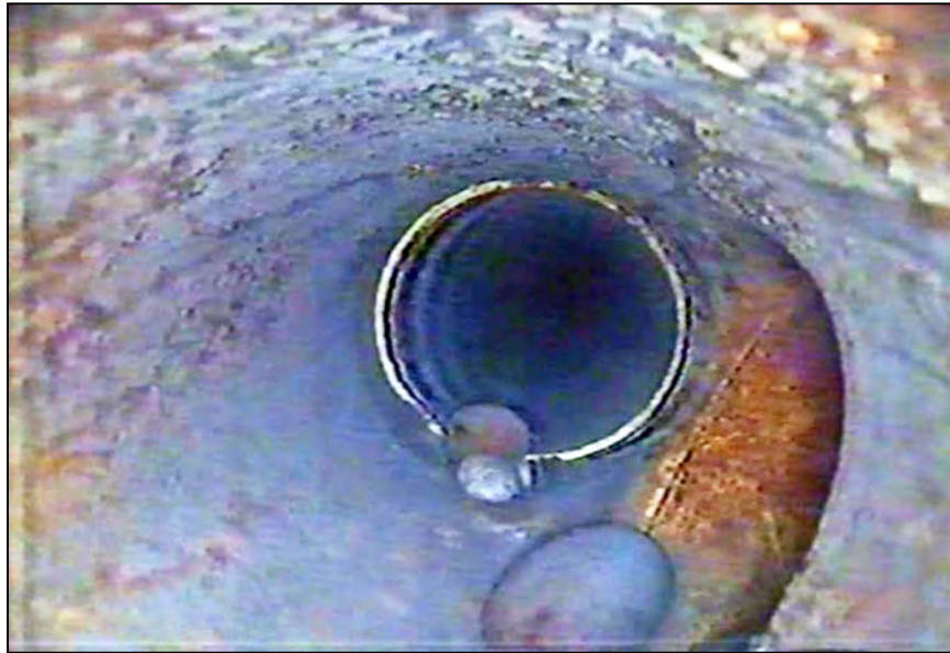
Figure A-110.—Isolated gravel in Underdrain No. 1 at T-intersection with pipe just downstream of second bend (location where pipe becomes horizontal).
