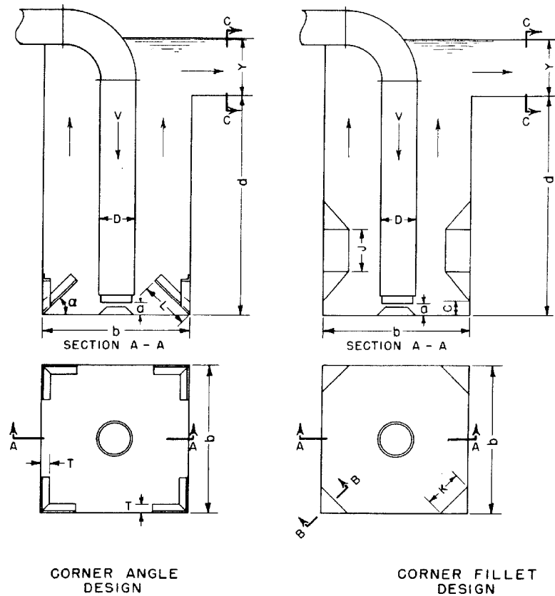
Figure 63.—Typical Reclamation stilling well application. The corner fillets and pedestal in the invert tend to maximize the circulation and energy dissipation in the lower portion of the well (Reclamation, 1973, p. 29). See Reclamation (1973) for information related to the variables as denoted in this figure.
