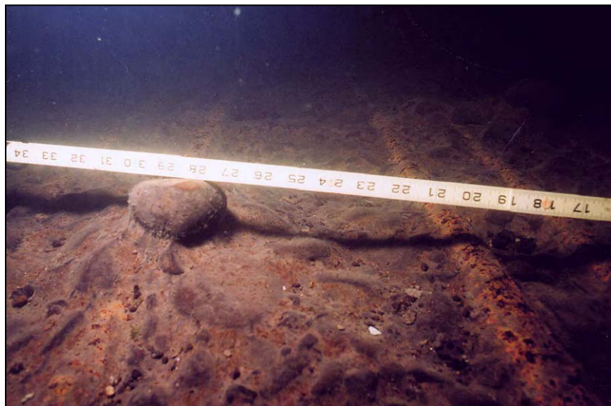
Figure A-12.—View of outlet works stilling basin showing 3-inch diameter aggregate still attached to concrete matrix. Erosion of floor is approximately 4 inches. Note exposed rebar on the right side of the photograph.
