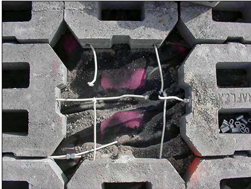
Figure 131.—Polyester cables.
