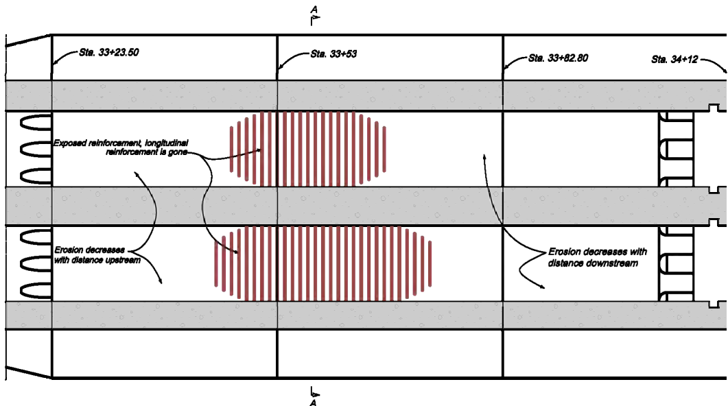
PLAN SECTION OF RIVER OUTLET WORKS STILLING BASIN (Cut near floor elevation)
