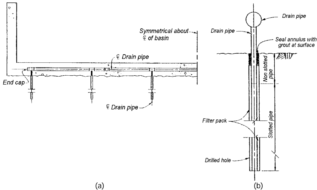
Figure 29.—Alternative underdrain system—(a) lateral (horizontal) collector drain with drilled/formed (vertical) weep hole drains. Note lateral collector drain is embedded in concrete to minimize disturbance to foundation. Cleanouts and covers for vertical drilled/formed drains are not shown, but are required for maintenance and inspection. (b) Typical detail of vertical drilled drain hole.
