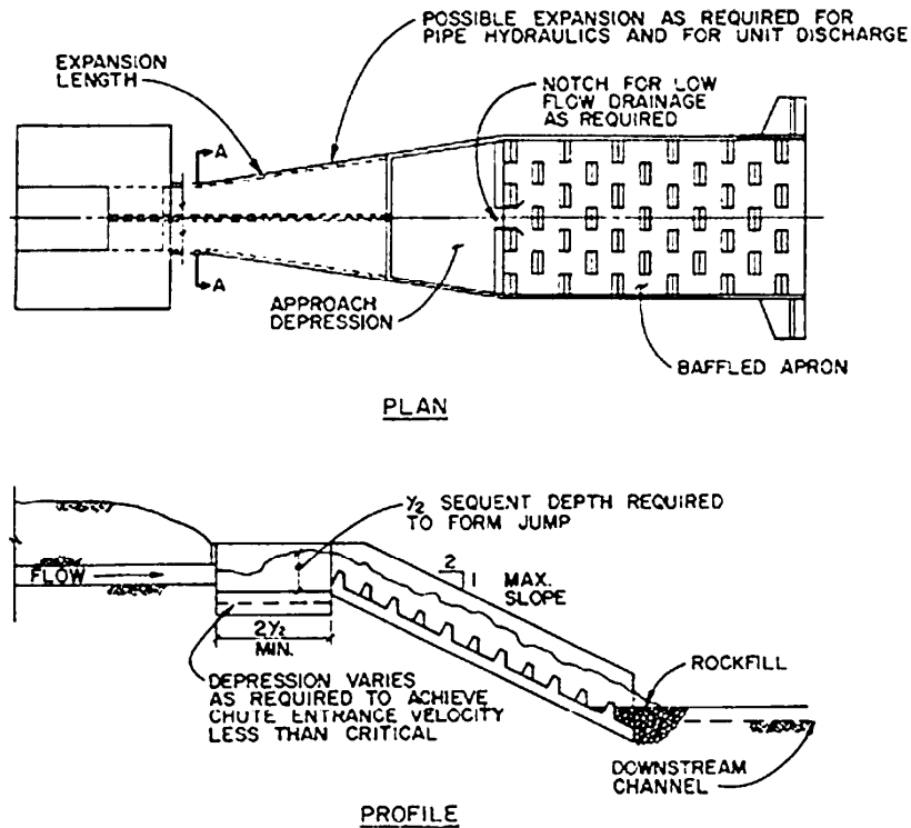
Figure 138.—Baffled chute with approach depression to lower approach velocities (Urban Drainage and Flood Control District, 2008, p. HS-76). See Urban Drainage and Flood Control District (2008) for information concerning the variables as denoted in this figure.
