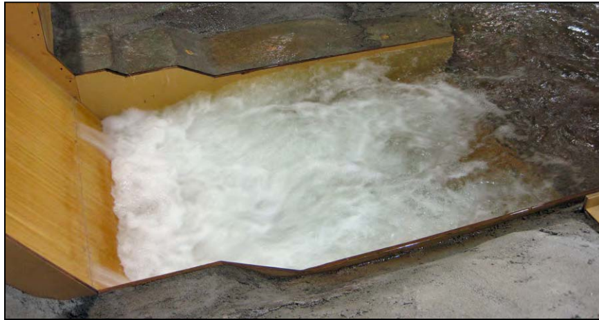
Figure 41. —This figure shows a hydraulic jump occurring in a 1:48-scale model of a type V stilling basin for a spillway. The operating condition equates to a prototype discharge of 60,000 ft 3 /s. The 242-foot wide stilling basin has an 0.8:1 slope for the upstream 178.7-foot length and is horizontal for the downstream 146.8-foot length. The stilling basin has a 15-foot high solid end sill. The figure most closely depicts the condition discussed in case C where the upstream toe of the hydraulic jump occurs on the slope and the downstream end of the jump is at the junction of the slope and the horizontal apron (for this example, where the break in floor slope goes from 0.8:1 to horizontal).
