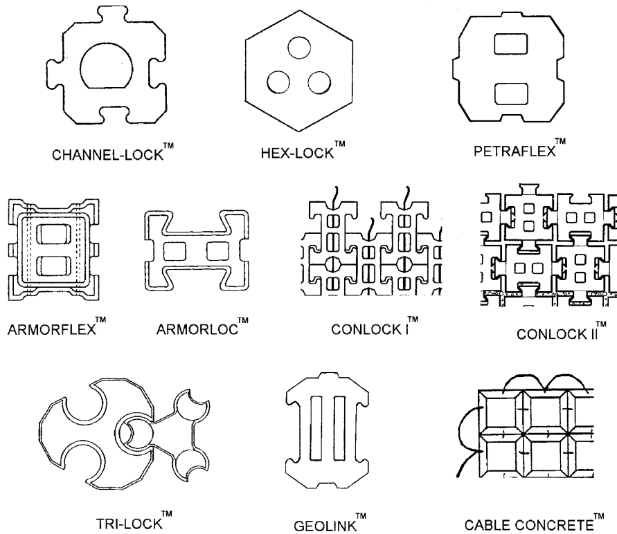
Figure 129.—Examples of ACB revetment systems Courtesy of HCFCD (2001) .
