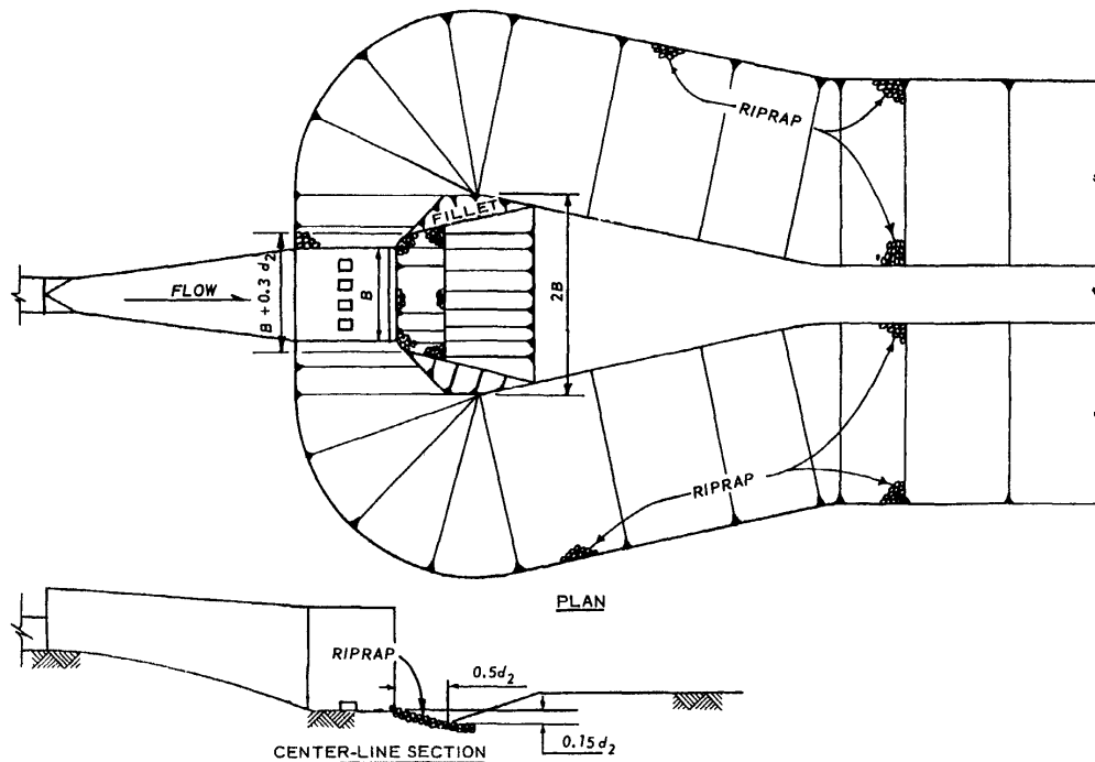
Figure 45.—Channel profile to prevent flow eddies leaving the USACE stilling basin from pulling downstream riprap into the stilling basin (USACE, 1980, p. C-43). See USACE (1980) for additional discussion of the information shown in this figure.
