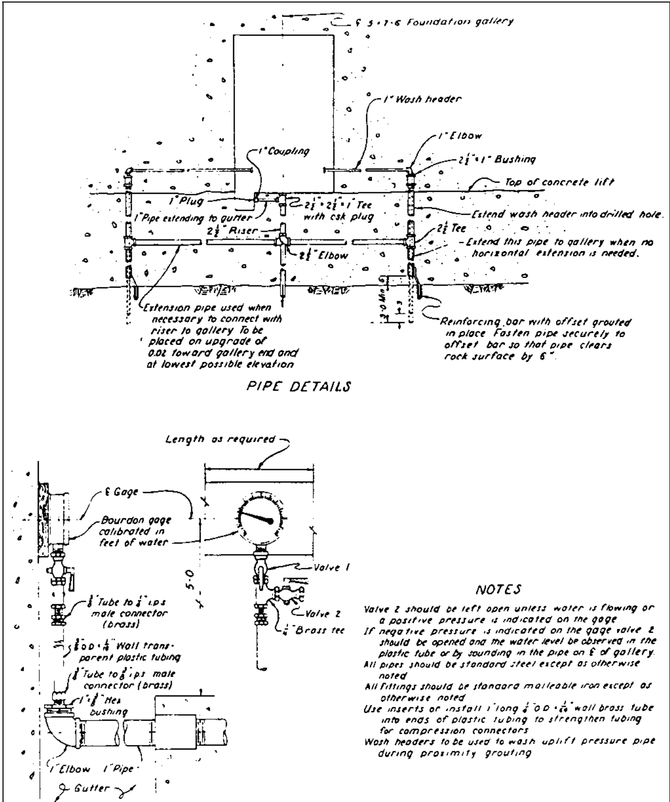
Figure 12-2. Typical Bourdon gauge installation (USBR 1987)
