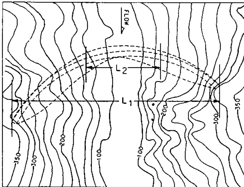
Figure 5-1. Determination of empirical values L_1 and L_2
