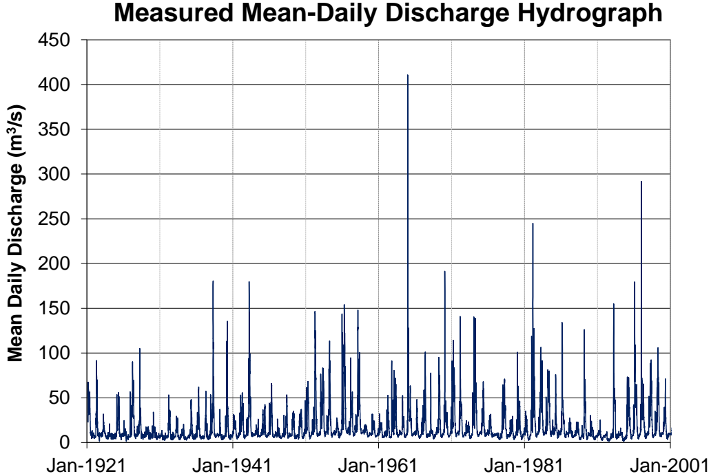
Figure 14.—Example mean-daily discharge history for the Sprague River in Oregon.
