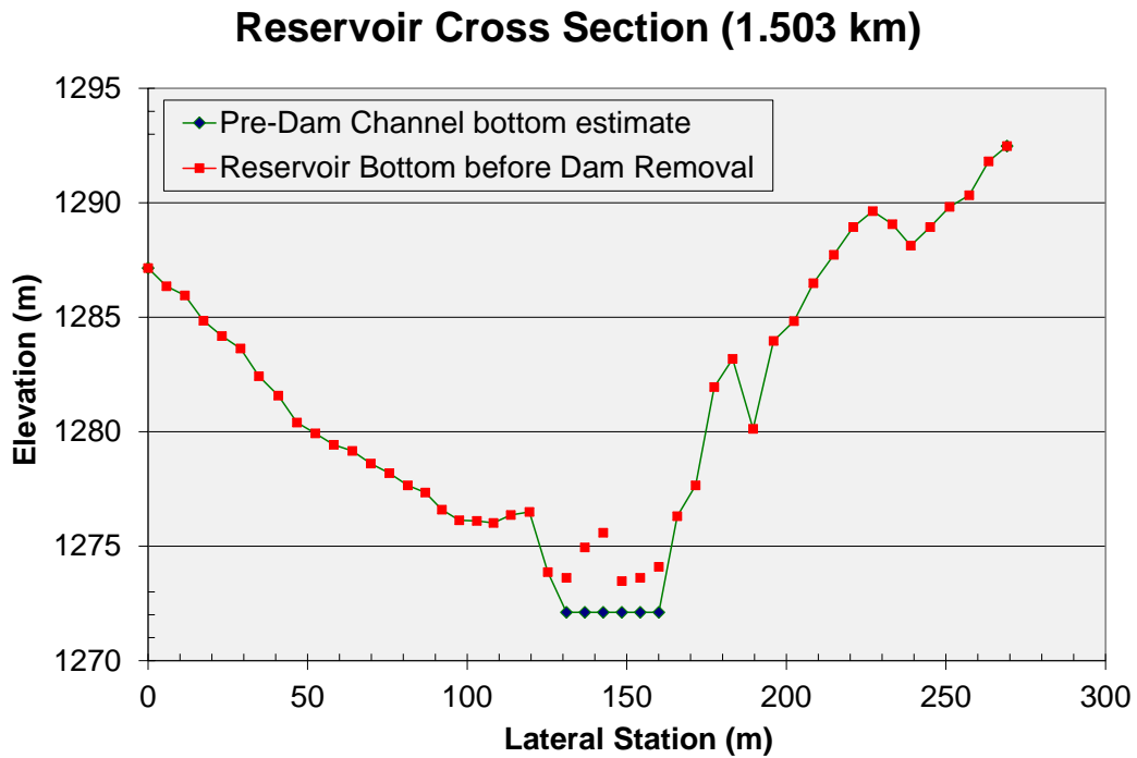
Figure 18.—Example reservoir cross section plot.
