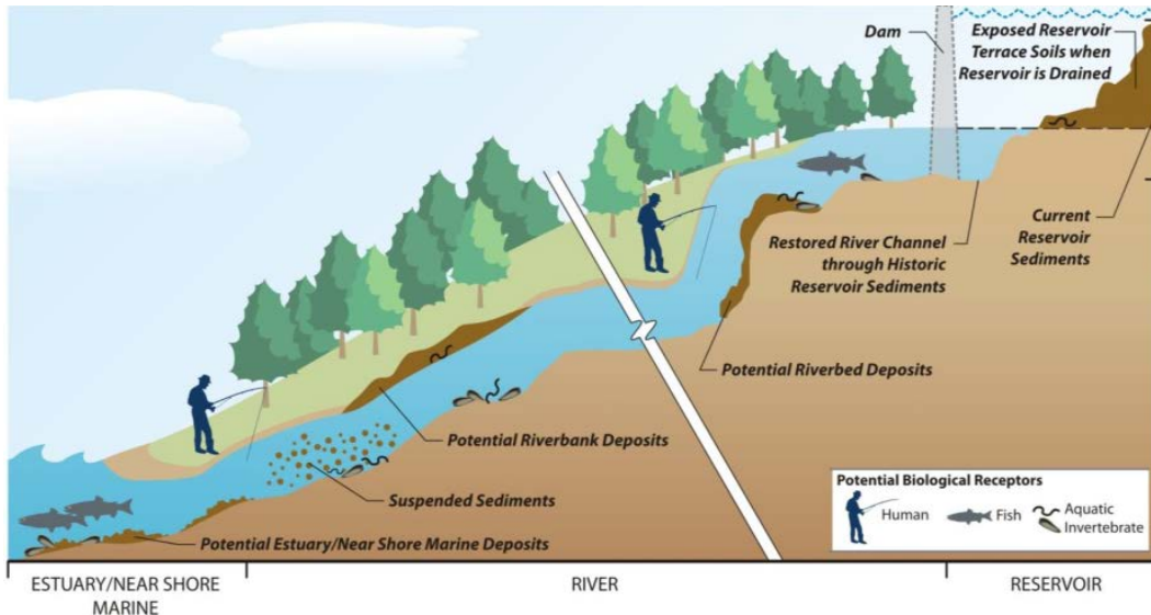
Figure 9.—Potential pathways of released reservoir sediment into downstream river channel utilized on Klamath River evaluation (CDM, 2011).
