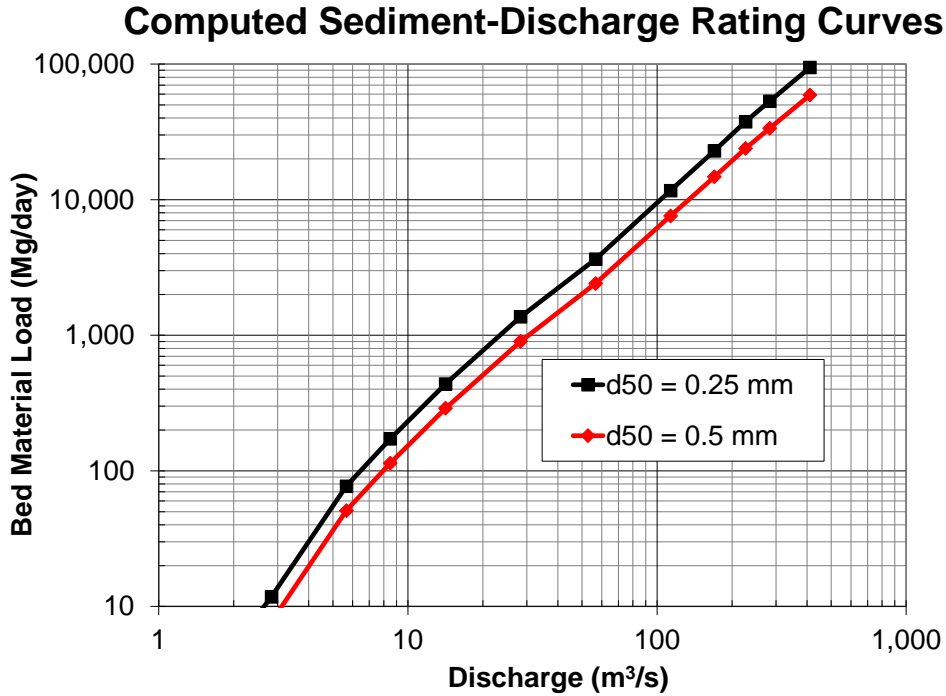
Figure 13.—Example sediment-discharge rating curves computed for the Sprague River in Oregon, using the sediment transport equation by Yang (1973) for sand, versus discharge for two different median sand sizes (0.25 mm and 0.5 mm).
