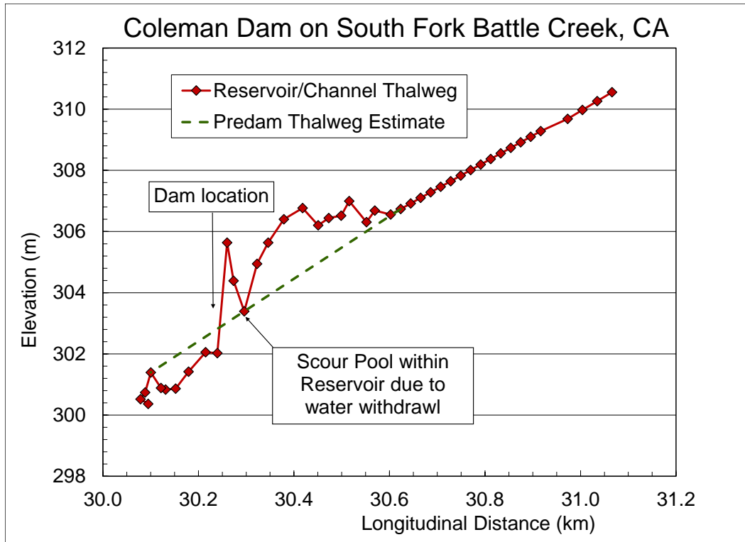
Figure 8.—Example estimate of the predam profile through reservoir sediments at Coleman Dam on South Fork Battle Creek, CA.
