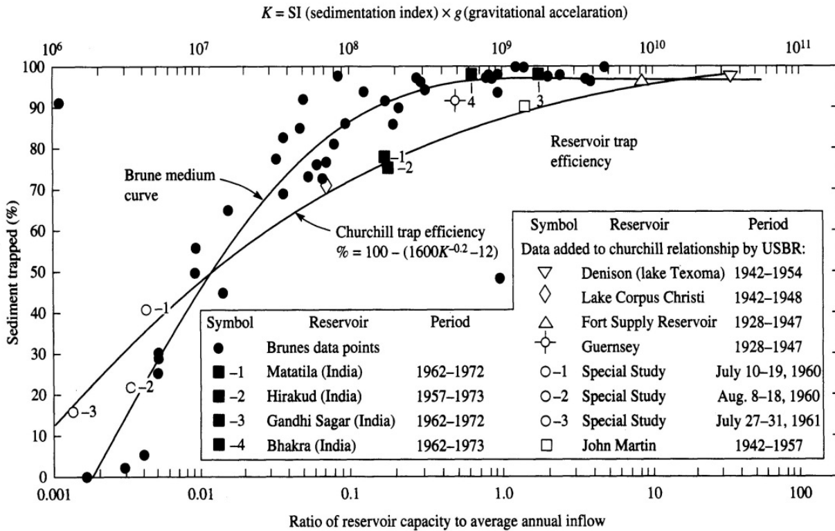
Figure A-6.—Empirical reservoir sediment trap efficiency curves based on Churchill (1948) and Brune (1953) and additional case studies (Strand and Pemberton, 1982).
