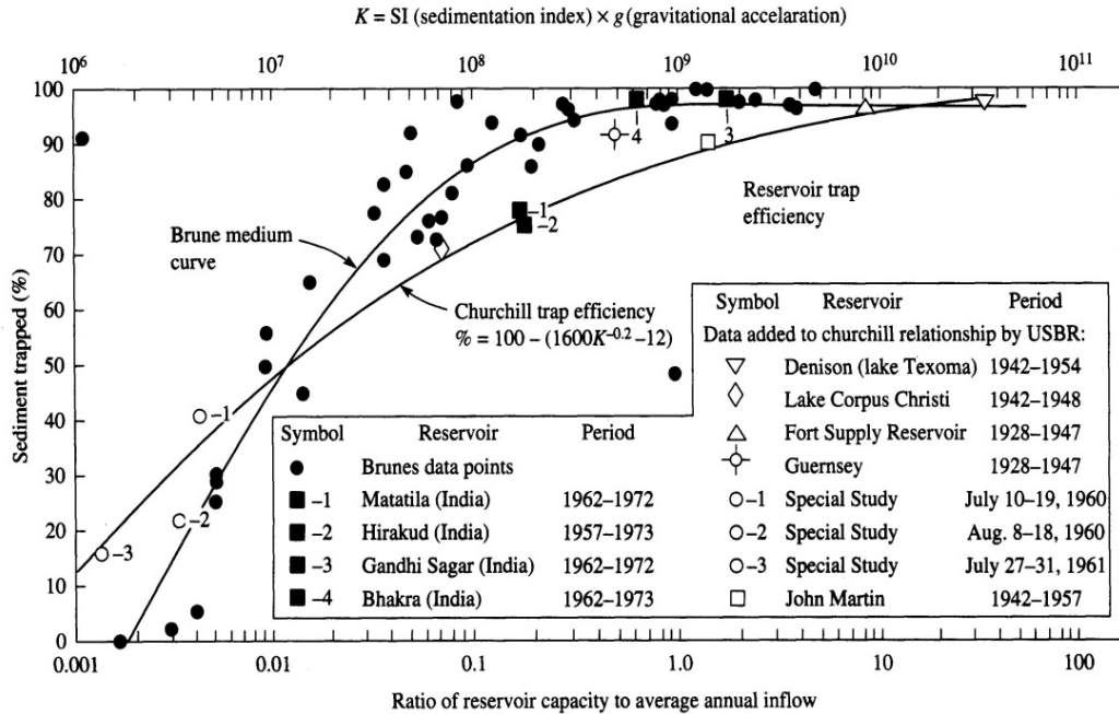
Figure 12.—Empirical reservoir sediment trap efficiency curves based on Churchill (1948) and Brune (1953) and additional case studies (Strand and Pemberton, 1982).
