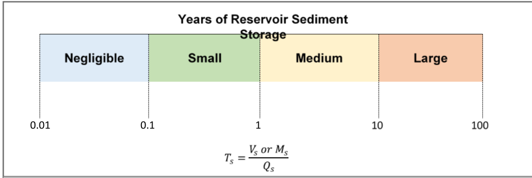
Figure 16.—Relative probability of sediment impact based on ratio of reservoir sediment volume or mass ( V_s ) to average annual sediment load ( Q_s ).
