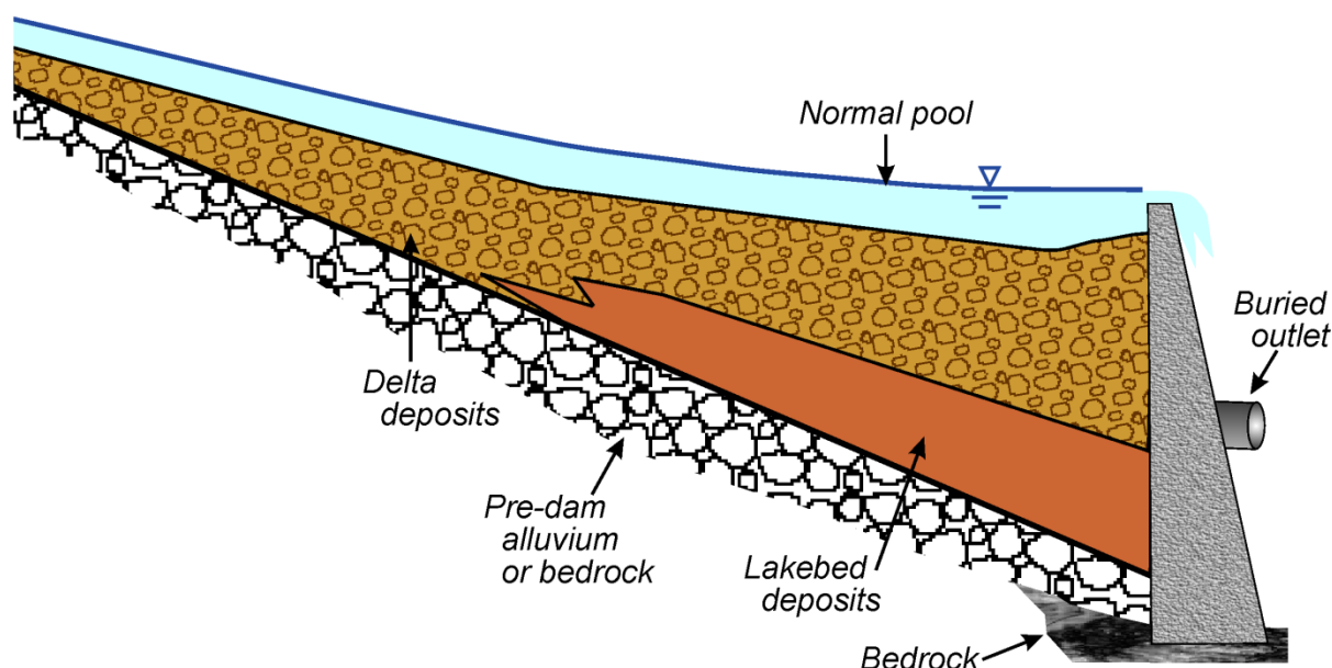
Figure A-7.—Reservoir sediment profile after the reservoir has filled with sediment.
