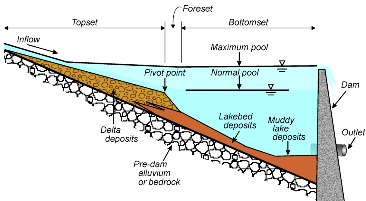
Figure A-1.—Reservoir sediment profile with delta and lakebed sediment deposits (after Morris and Fan, 1997).
