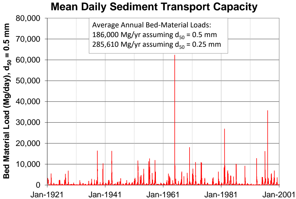
Figure 15.—Example daily coarse sediment load hydrograph computed for the Sprague River in Oregon.
