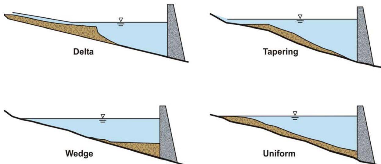
Figure A-3.—Four basic patterns of reservoir sediment deposition: delta, tapering, wedge, and uniform (Morris and Fan, 1997).
