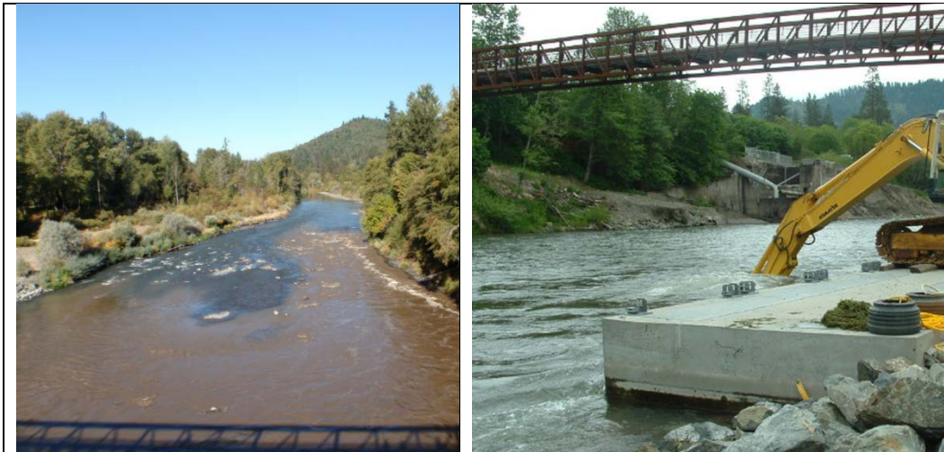
Figure 34.—Downstream view of short-term turbidity plume released from breaching of Savage Rapids Dam in Oregon (left photo) and view of sediment excavation at water intake just downstream of dam (right photo). Photo taken by Jennifer Bountry, Bureau of Reclamation.
