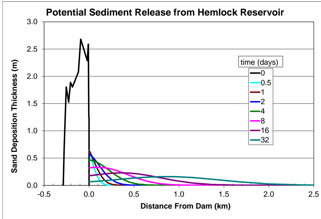
Figure 28.—Example sediment wave model results for the removal of Hemlock Dam on Trout Creek in southwest Washington State.
