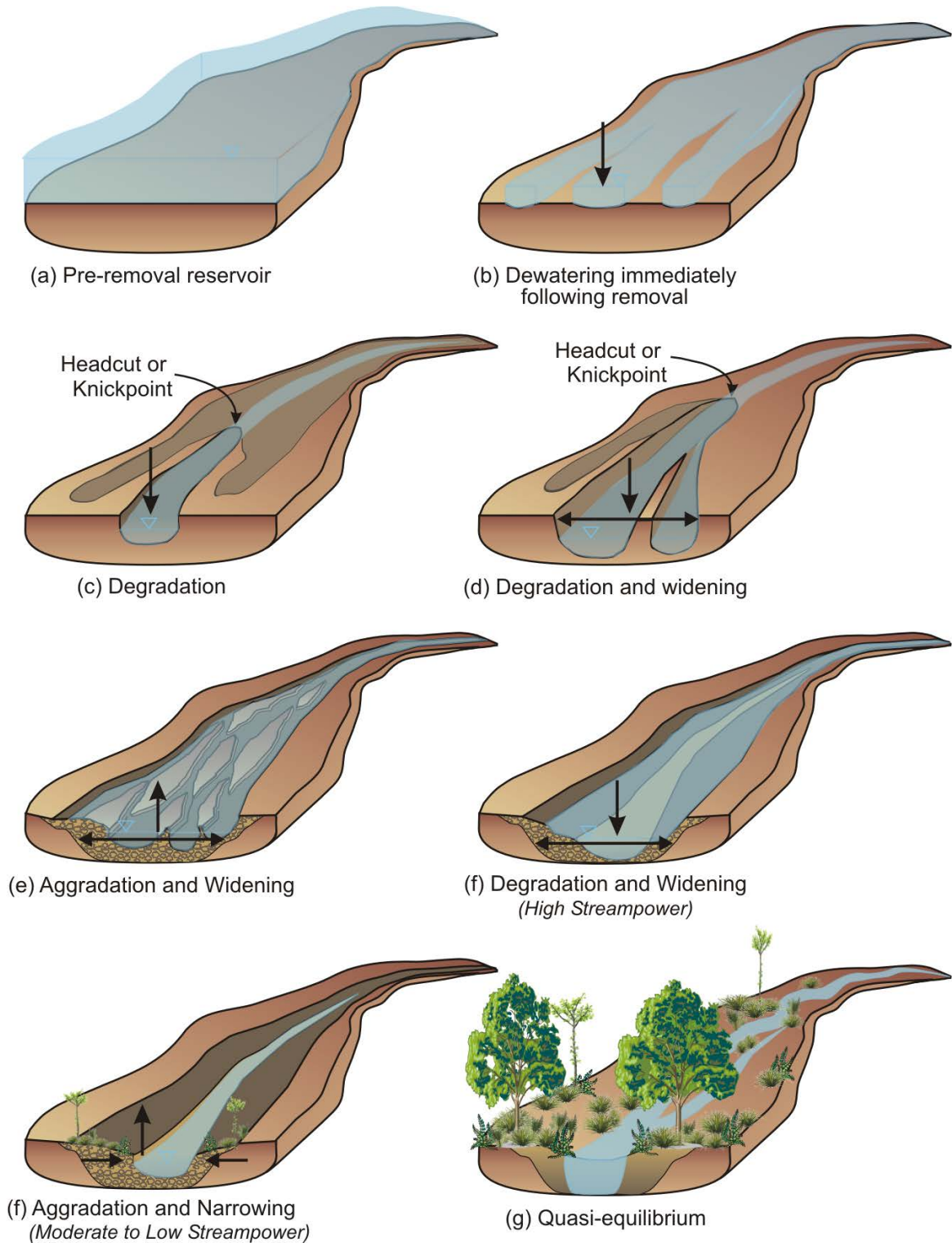
Figure 25.—Conceptual model of sediment erosion from the reservoir modified from Doyle et al. (2003a) and Cannatelli and Curran (2012).
