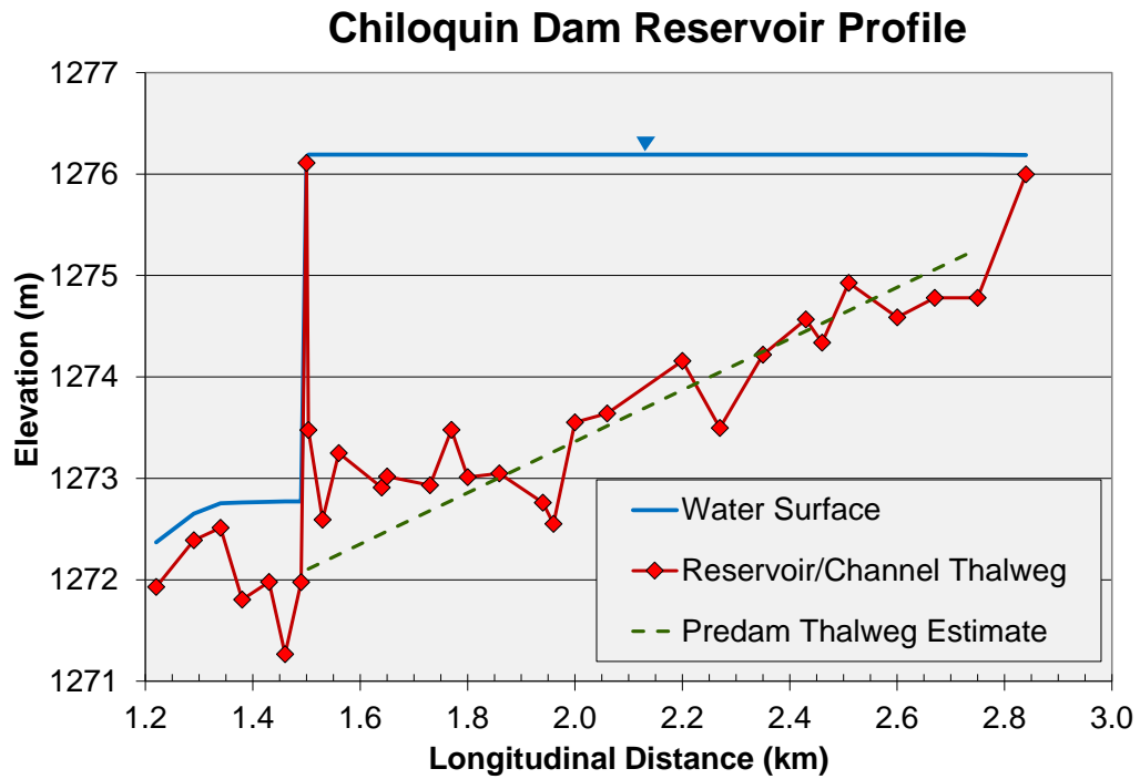
Figure 17.—Longitudinal profiles of the reservoir behind Chiloquin Dam.
