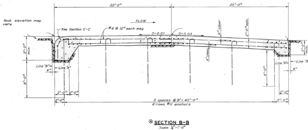
Spillway Control Sill Detail (As-Built Drawings)
