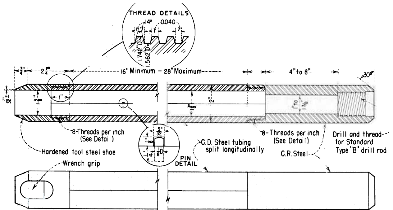
Figure 5-42. Standard split-barrel sampler. 101-D-169.
