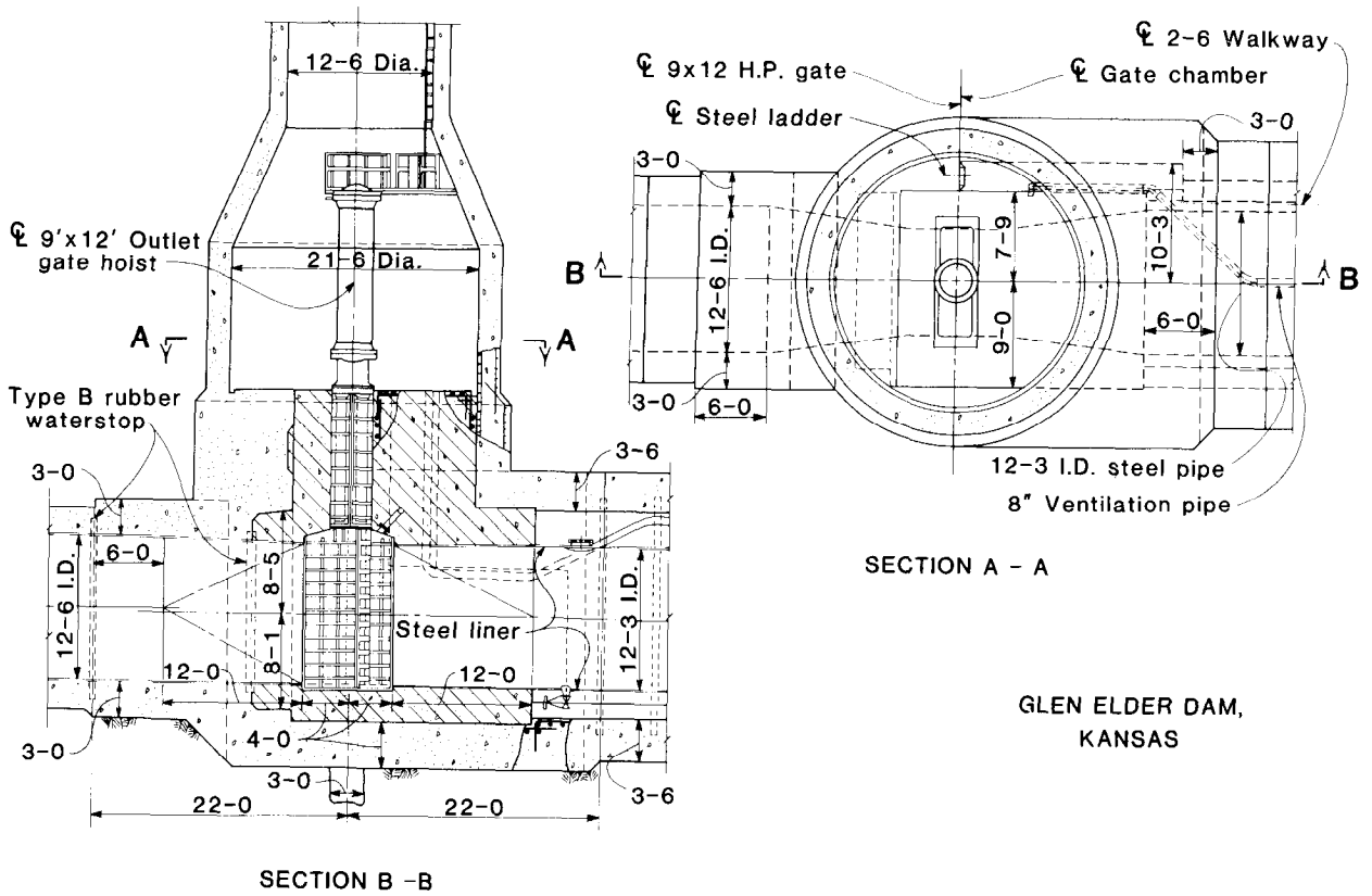
Figure 10-32.—Gate chamber and shaft with high-pressure gates. 103-D-1846.
