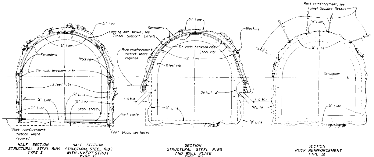
TYPICAL TUNNEL SUPPORT SECTIONS (MODIFIED HORSESHOE TUNNELS)
