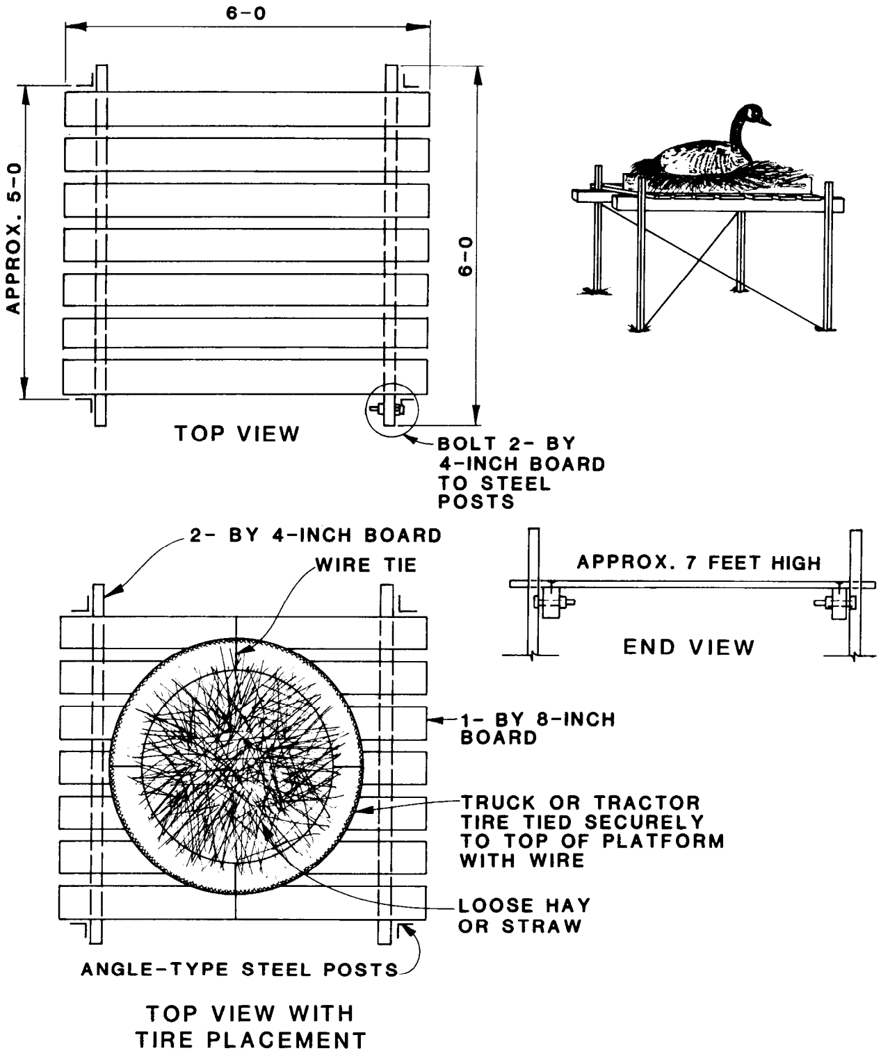
Figure 2-8.—Details for constructing a goose-nesting platform. From [14]. 103-D-1798.
