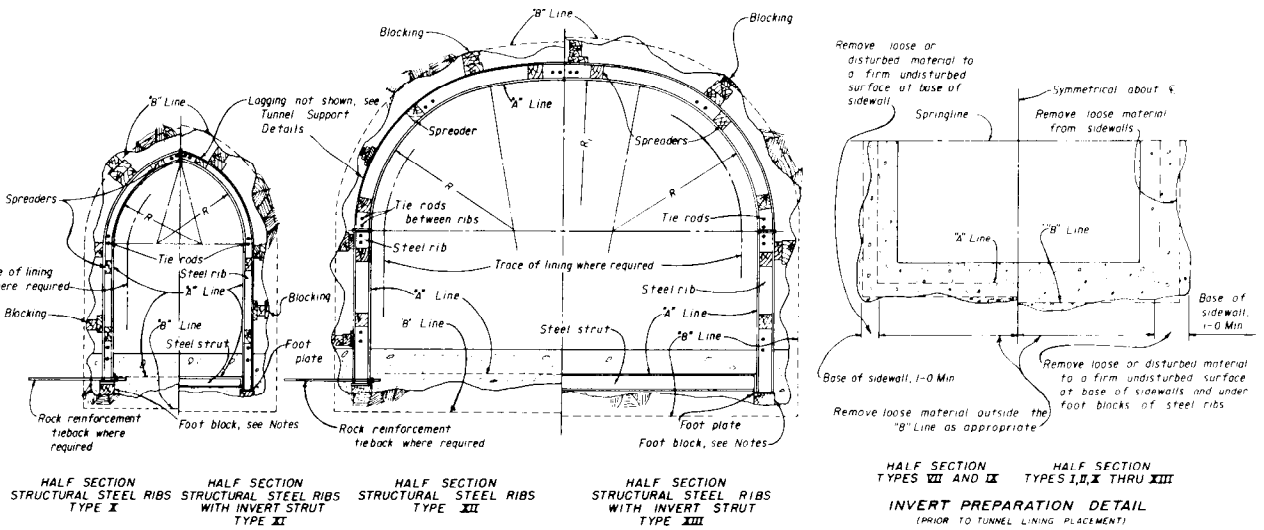
TYPICAL TUNNEL SUPPORT SECTIONS (MISCELLANEOUS TUNNELS)
