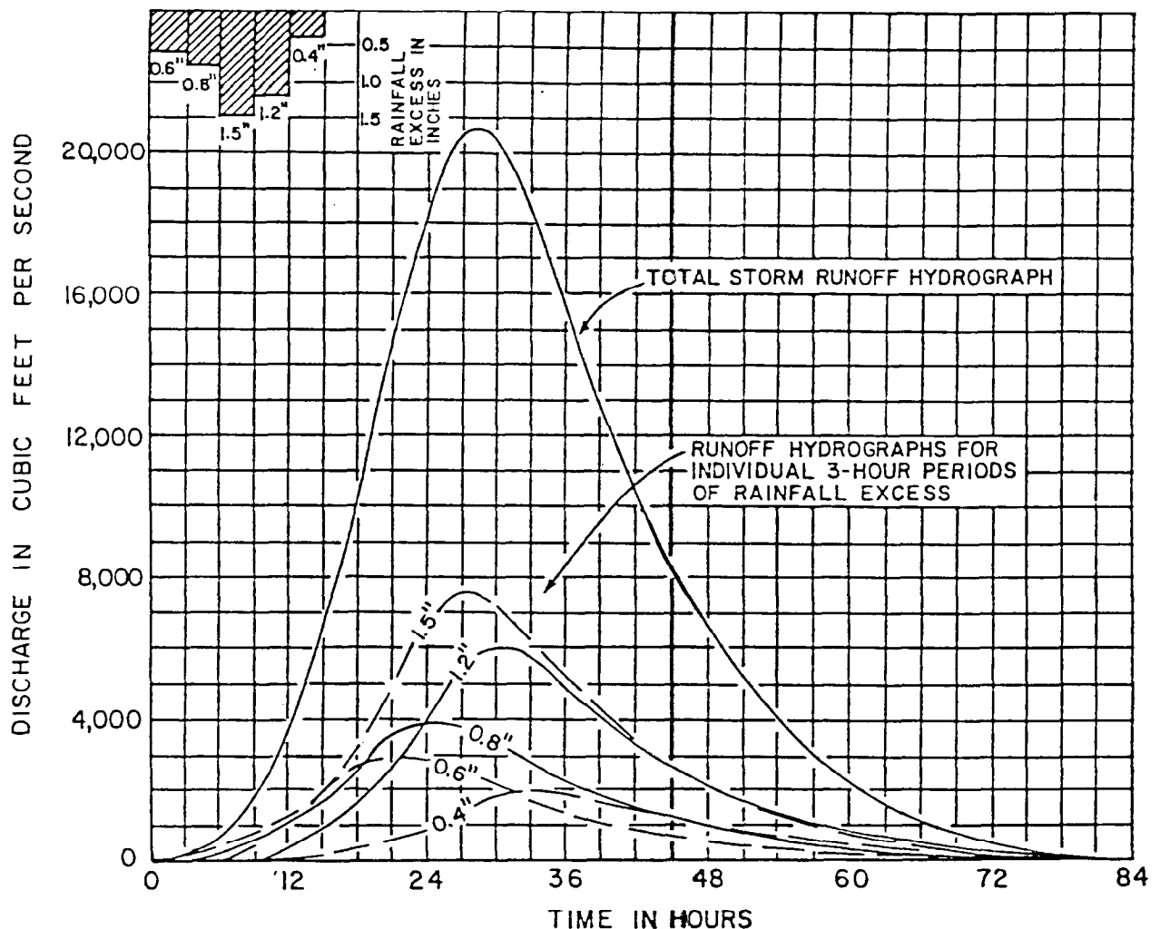
Figure 3-2.—Unit hydrograph application. 103-D-1849.
