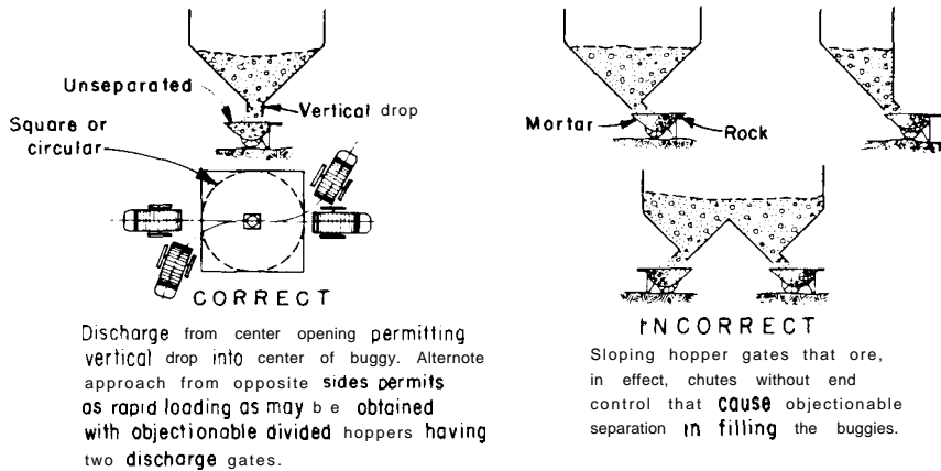
Figure F-1 2.—Methods of handling concrete with buckets, hoppers, and buggies. PX-D-25316.
