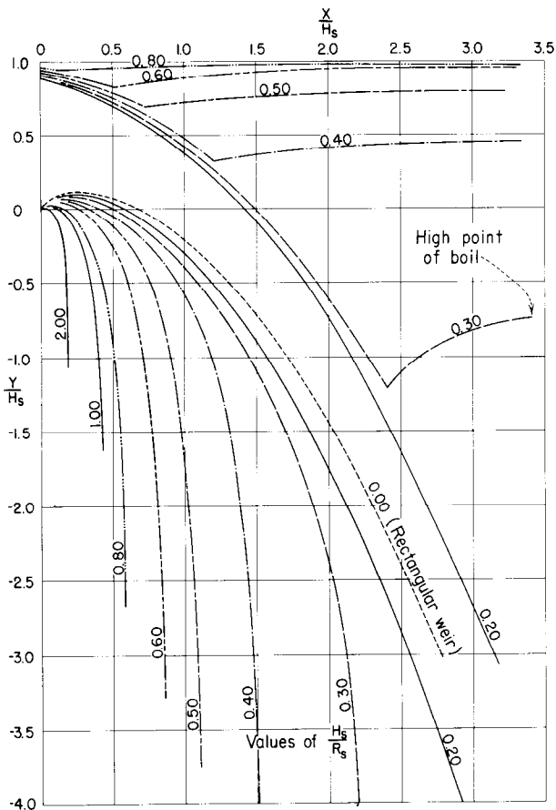
Figure 9-60.—Upper and lower nappe profiles for circular weir (aerated nappe and negligible approach velocity). 288-D-2444.
