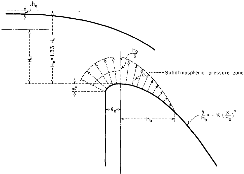
Figure 9-29.—Subatmospheric crest pressures for H_c/H_0 = 0.75 . 288-D-2415.
