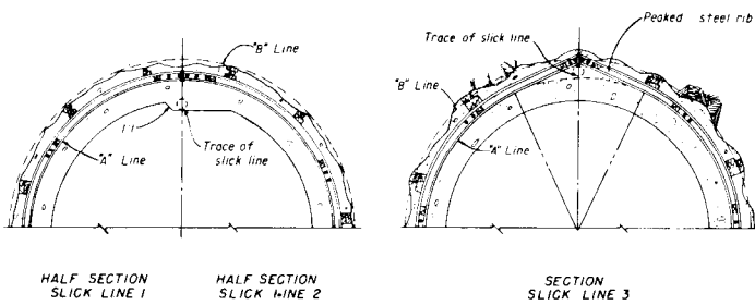
METHODS TO ACCOMMODATE SLICK LINE
