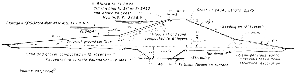
Figure 6-66.—Dickinson Dam. Located on the Heart River, North Dakota (constructed 1948-50). From 103-D-584.
