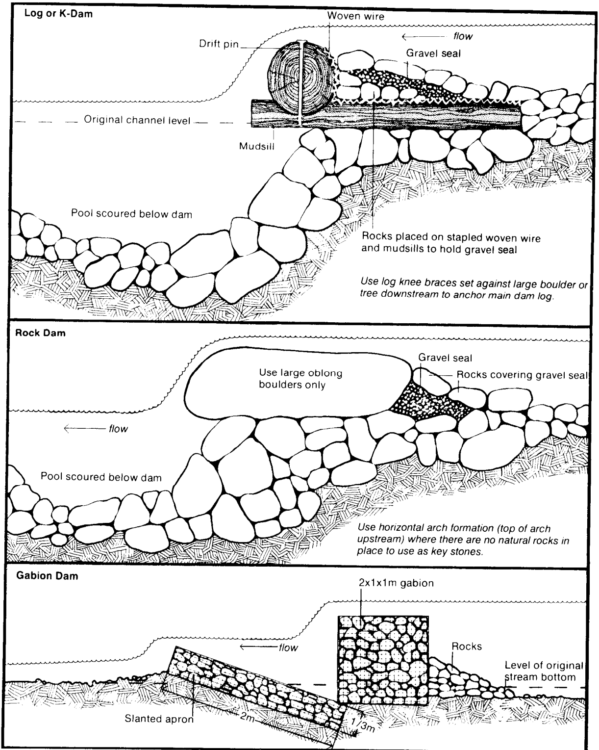
Figure 2-1.—Several types of check dams. Scour holes developed by these dams create habitat conditions that increase fish populations. 103-D-1793.
